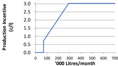
Chart below shows approximate c/l production incentive -v- monthly production (assumes reference composition)
